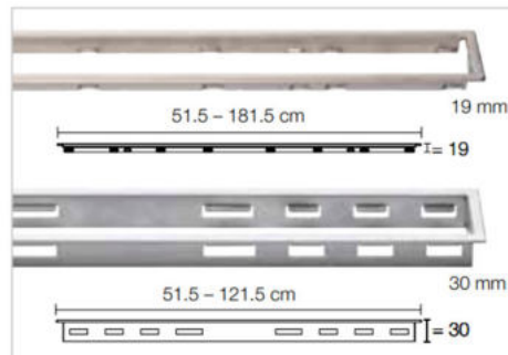
Schlüter®-KERDI-LINE-B
